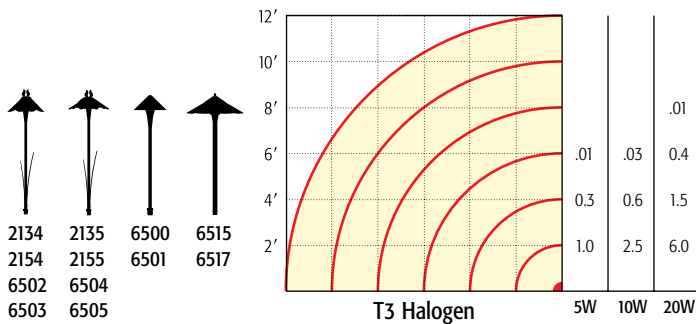
Horizontal Foot Candle Quarter Spread
