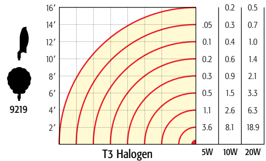
Vertical Foot Candle Quarter Spread
